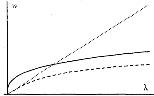
Figure 1. Eq (10) (solid line) compared to the \lambda -dependence of the 1D-step model (dashed) and its linear approximation (dotted).
