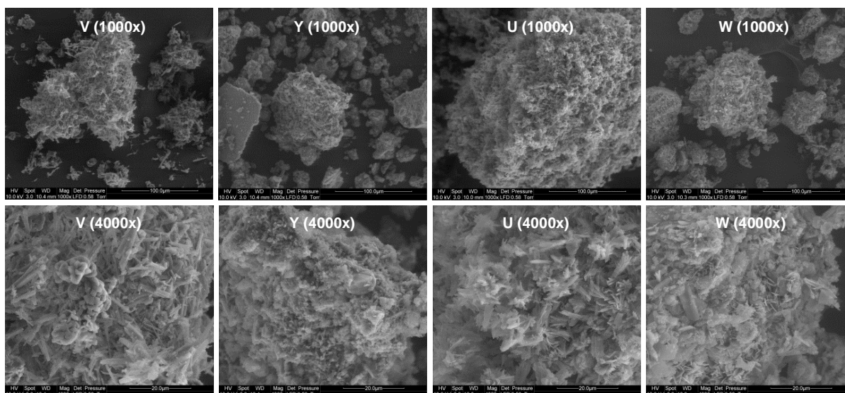
Figure 3. Scanning electron micrographs of NRB V, Y, U and W; at 1000 \times and 4000 \times magnification.
