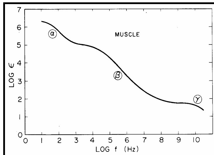
Figure 7: The dielectric constant of muscle as a function of frequency, Schwan and Foster (1980).
