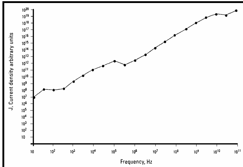
Figure 8: Capacitive induced current density in a toroid of human muscle tissue of unitary radius, exposed to a unitary magnetic field induction, Vignati and Giuliani (1997).
