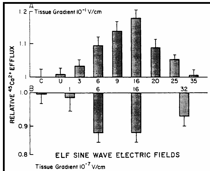
Figure 9: Relative \text{Ca}^{2+} efflux (positive and negative) from isolated chick cerebral hemisphere exposed to (A) weak RF field (147 MHz, 0.8 \text{ mW/cm}^2 , 56 V/m in air), amplitude modulated at low frequencies (abscissa) and (B) ELF electric field (56 V/m in air) over the same ELF modulation frequencies, Adey (1988).
