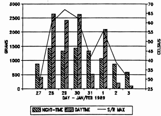
Figure 3.24 Net water evaporation proportioned between night-time and day time evaporation.
