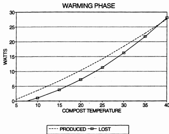
Figure 4.34 The heat produced Q_{\text{gain}} and heat lost Q_{\text{T}} plotted against compost temperature - Warming phase.
