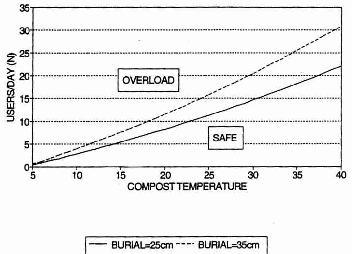
Figure 4.39 The effect of compost temperature on number of users before overload conditions occur. Based on the Soltran toilet.
