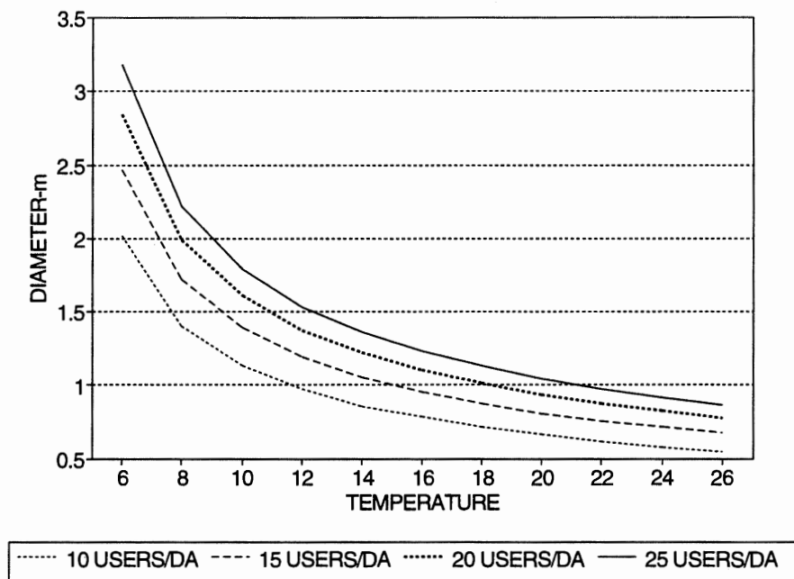
Figure A.3.2 The effect of temperature and usage rate on vault size (assuming a circular drum is used)
