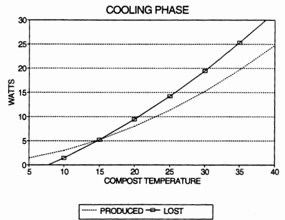
Figure 4.35 The heat produced Q_{\text{gain}} and heat lost Q_{\text{T}} plotted against compost temperature - Cooling phase.
