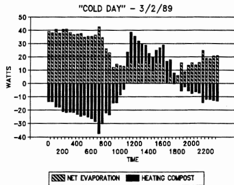
Figure 3.16 The energy transferred to the compost room - cold day
