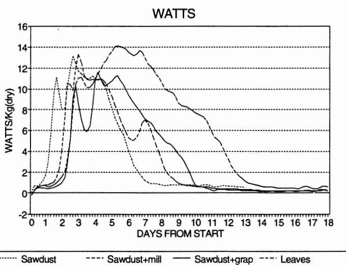
Figure 4.18 The effect of different bulking materials on the composting process - WARM ROOM
