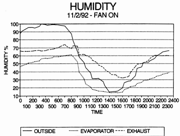
Figure 3.20 The effect of the fan on humidity within the Soltran. Compare to figure 3.6.
