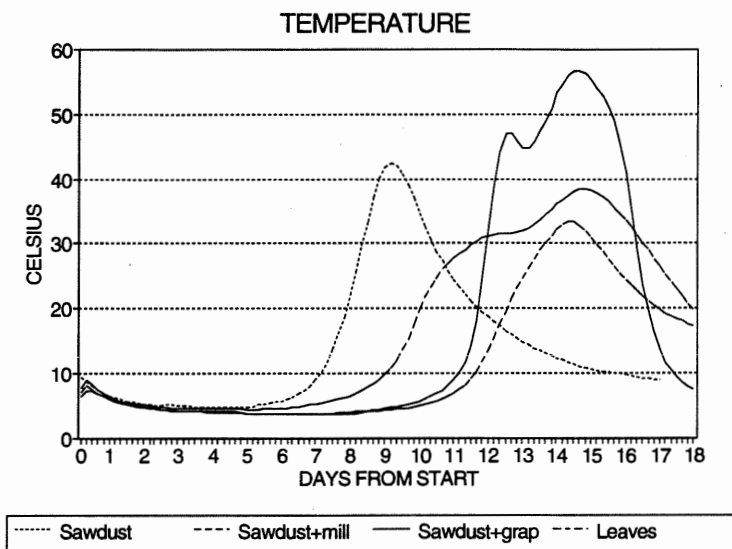
Figure 4.19 The effect of different bulking materials on the composting process - COLD ROOM
