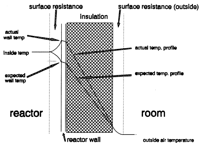
Figure A.1.1 Temperature profile through the wall of the compost reactor.
