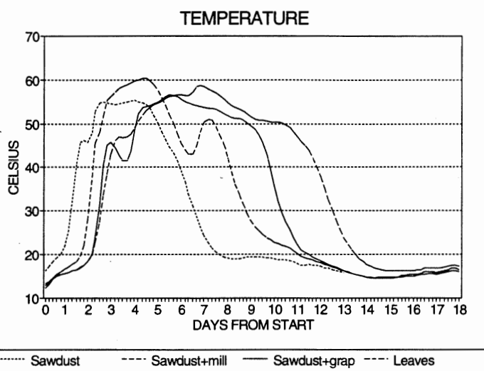
Figure 4.17 The effect of different bulking materials on the composting process - WARM ROOM
