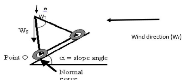
Figure 1. Centre pivot at an inclined surface
