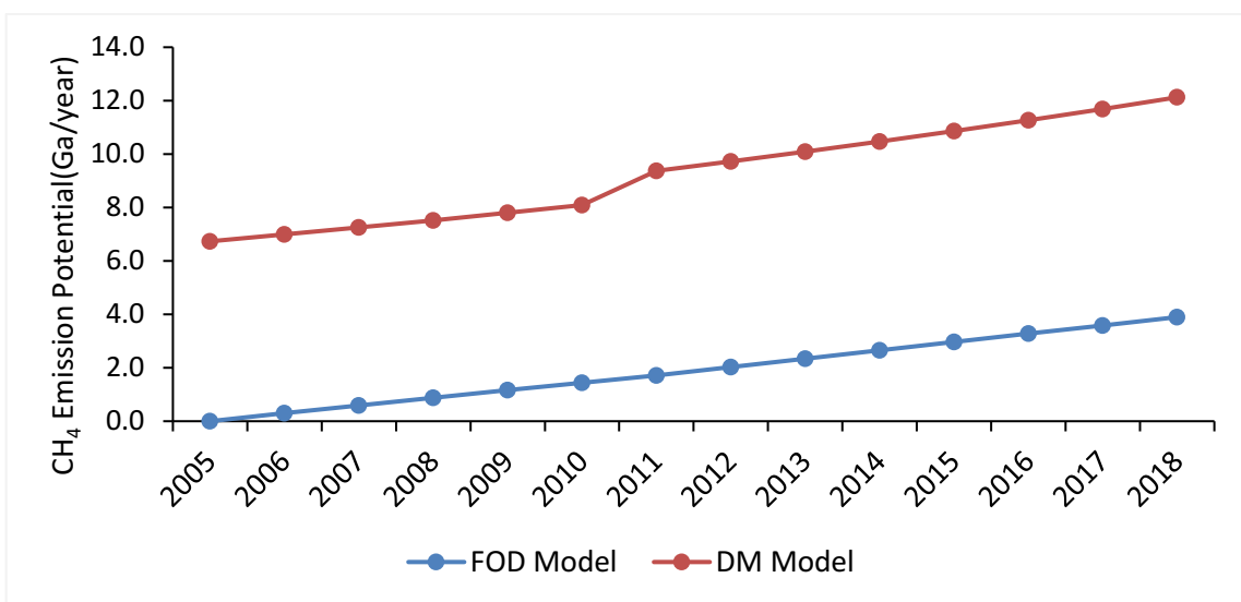
Figure 4-7: Methane emissions in Sisdole landfill site using various models.
