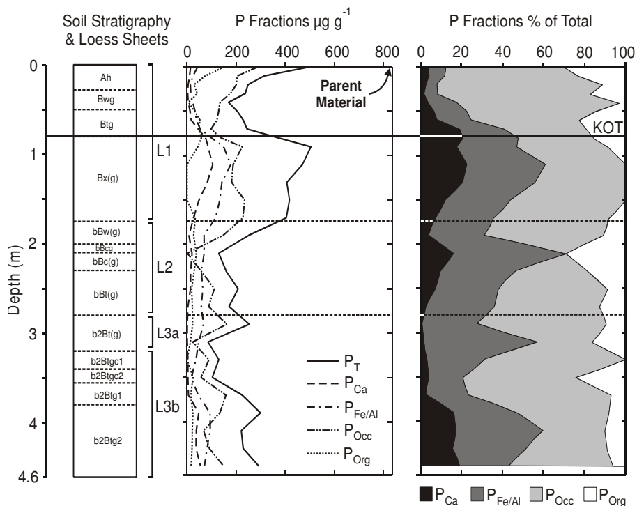
Figure 1. Phosphorus fractions presented as absolute values (centre) and percentages of total values (right). Soil stratigraphy and loess sheet delineations are presented on the left. P_T = total P, P_{Ca} = apatite P, P_{Fe/Al} = Fe- and Al-bound P, P_{Occ} = occluded P, P_{Org} = occluded P. Also shown is the value ( P_T ) of river silt parent material, and the stratigraphic location of the ca. 27 ka Kawakawa/Oruanui Tephra (KOT; solid line). Figure reproduced from Hughes et al. (2010) (in prep.).
