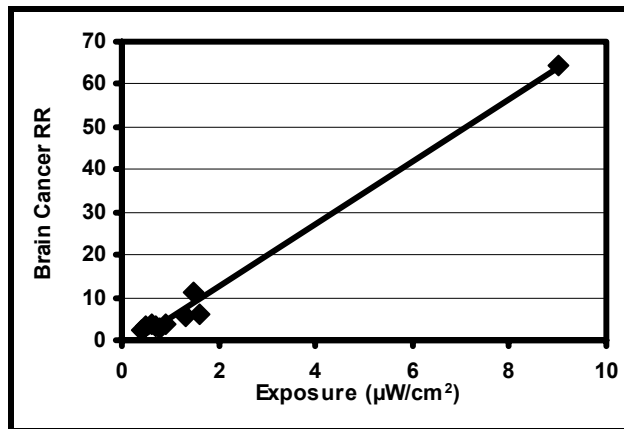
Figure 47: Childhood Brain Cancer as a function of measured and estimated RF/MW exposure in 0.5 km radial rings. Trend p < 0.00001 .
