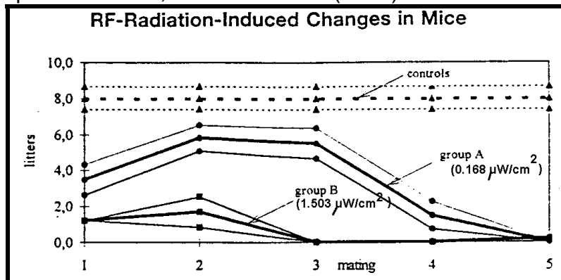
Figure 65: Reproductive rates in two groups of mice exposed to extremely low intensity radio signals, showing a dose response in the time taken to achieve full infertility of 3 matings for 1.503\mu\text{W}/\text{cm}^2 and 5 matings for 0.168\mu\text{W}/\text{cm}^2 .
