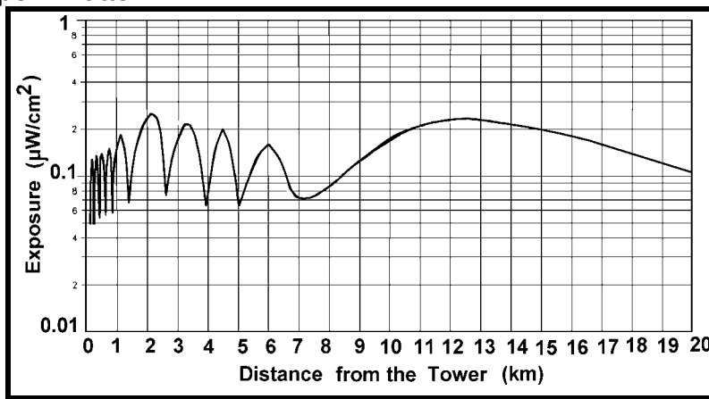
Figure 51: Ground level exposure for a typical UHF TV broadcast signal, from an antenna pattern from Hammett and Edison (1997), for a 18 MW EIRP transmitter at 460m AGL, for a flat surface.
