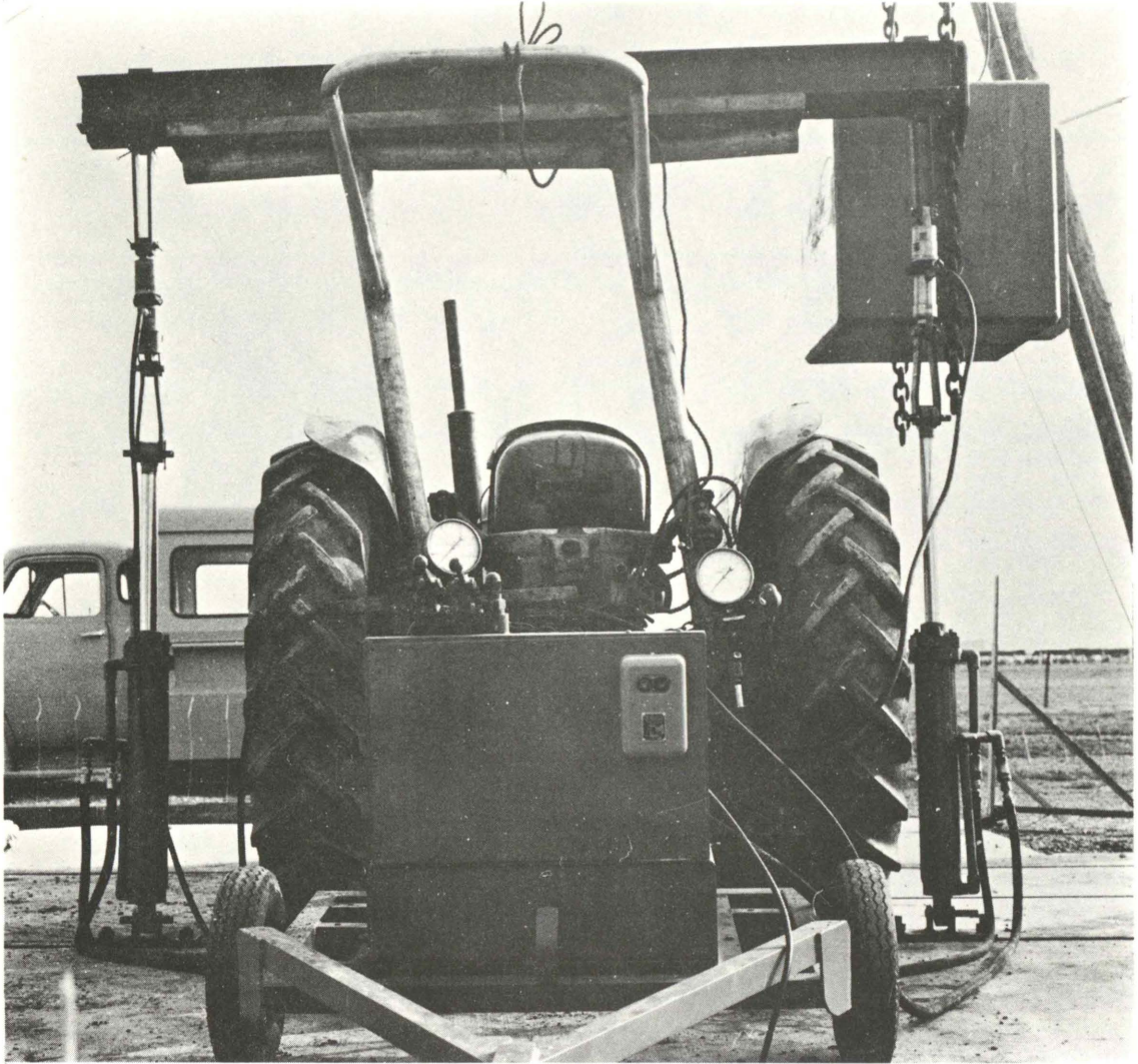
METHOD OF APPLYING CRUSHING LOAD TO SAFETY FRAME.
