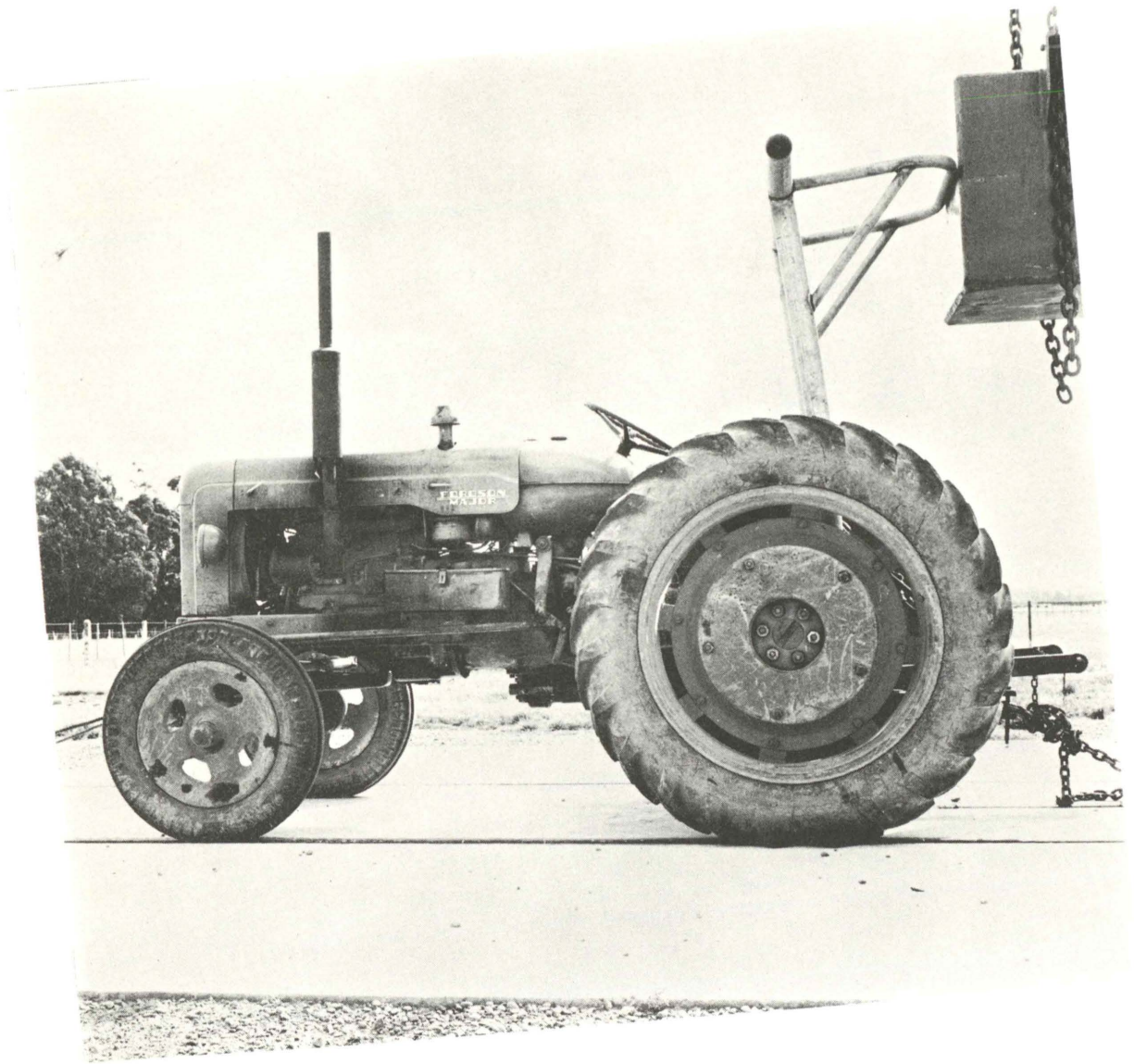
SAFE "T" SAFETY FRAME AFTER IMPACT FROM REAR.
