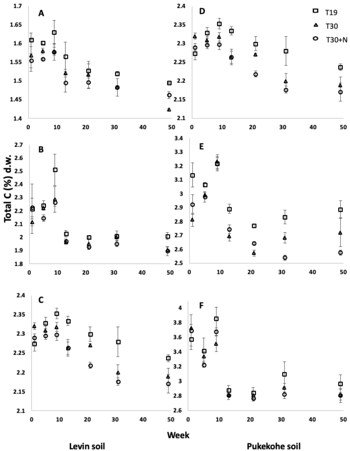
Figure 1. Changes of total C (C T ) in soils with time in treatments T-19, T-30, and T-30+N ((A) Levin soil control, (B) Levin soil + MC, (C) Levin soil + SC, (D) Pukekohe soil control, (E) Pukekohe soil +MC, (F) Pukekohe soil +SC). Error bars represent the standard error of the mean (n = 3).
